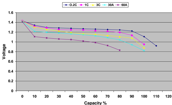
Discharging Curve
