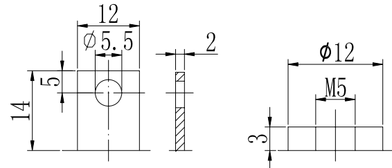
Terminal T3
