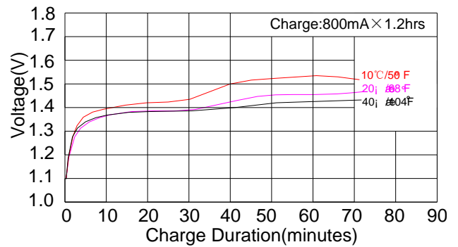
Rapid charge characteristics
