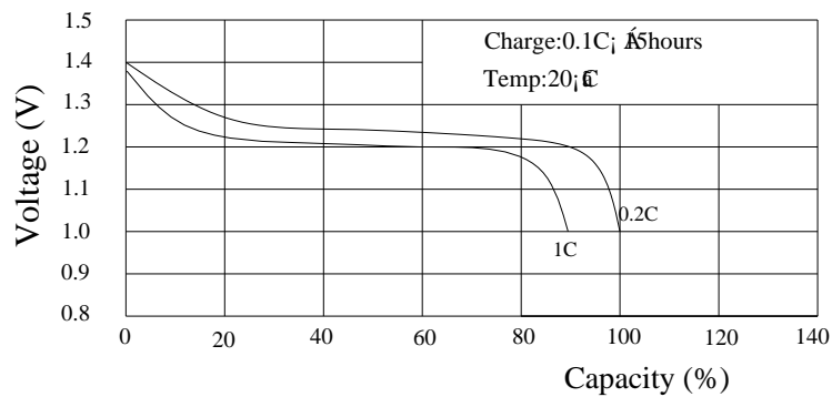
Discharge characteristics
